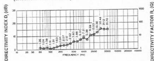
FIGURE 4 — TL12-1 One-Third-Octave Directivity vs Frequency (anechoic environment)
